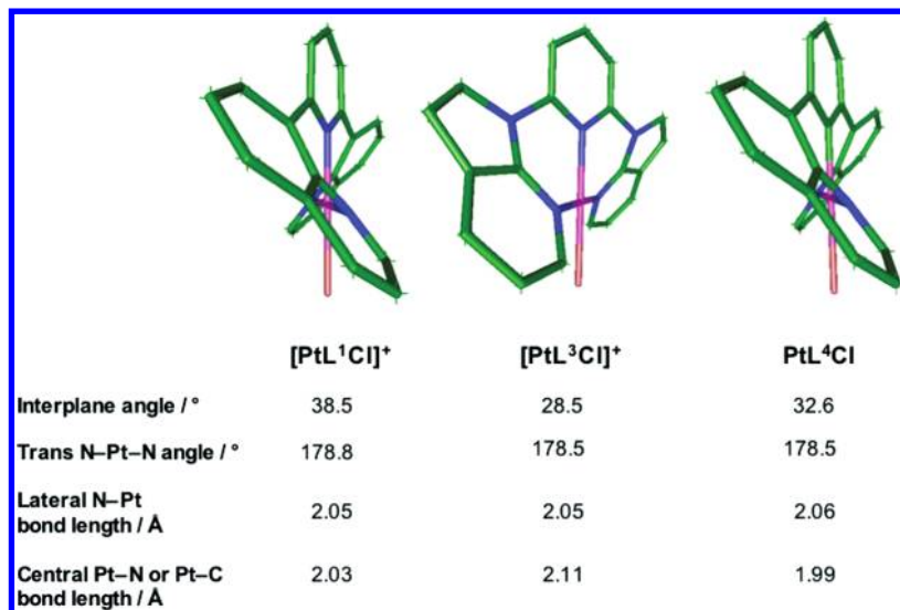
Figure 3. Structures of complexes [PtL 1 Cl] + , PtL 4 Cl, and [PtL 3 Cl] + predicted by energy minimization using DFT (gas-phase at 0 K), with the viewing angle selected to best reveal both the twist in the ligand and the planarity at the metal ion. The angle between the planes of the quinoline/azaindole rings and the central pyridine/benzene ring is given, together with the N–Pt–N angle for trans -related N atoms. Corresponding angles for [PtL 1 OMe] + are 31.6° and 174.9°, and for [PtL 1 (C≡C-tfp)] + 34.1° and 179.7°. Key bond lengths are also indicated.
