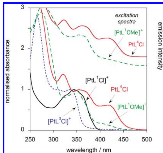
Figure 5. Normalized UV–visible absorption spectra of the Pt(II) complexes in \text{CH}_2\text{Cl}_2 at 298 K. The spectra of [\text{PtL}^1(\text{C}\equiv\text{C-tfp})]^+ and [\text{PtL}^2\text{Cl}]^+ are omitted here for clarity; they are provided in Figure S4 of the Supporting Information, and data is summarized in Table 2. Inset: excitation spectra of [\text{PtL}^1\text{OMe}]^+ and \text{PtL}^4\text{Cl} ( \lambda_{\text{em}} = 600 \text{ nm} ) in \text{CH}_2\text{Cl}_2 at 298 K.
