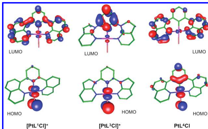
Figure 4. Frontier orbitals of complexes [PtL 1 Cl] + , [PtL 3 Cl] + , and PtL 4 Cl calculated by TD-DFT.
